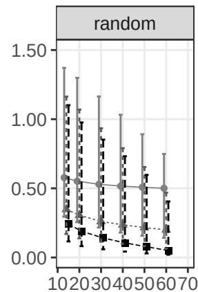
(C) RMSE
